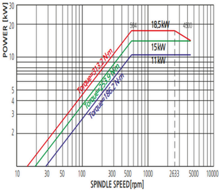
SL 2500 Y series (A Type)
