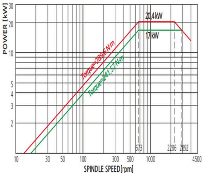
SL 2500 Y series (A Type)
