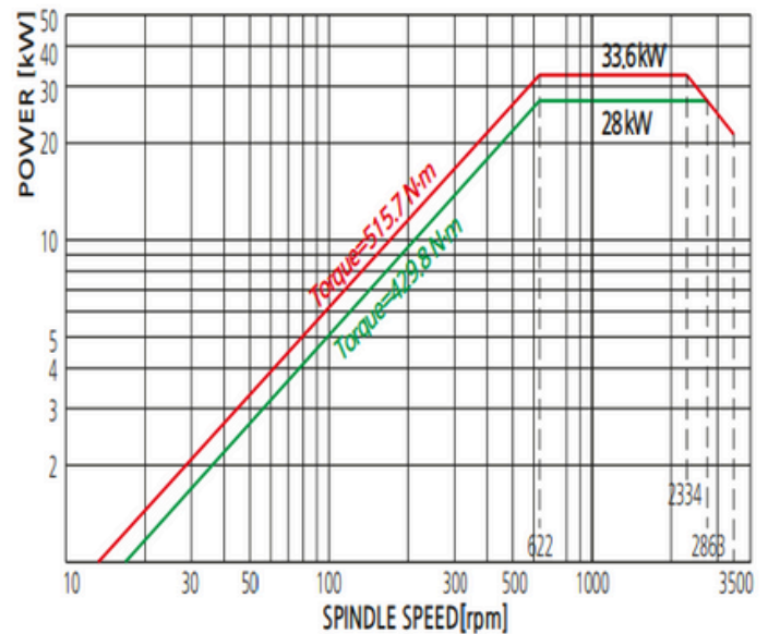
SL 2500 Y series (B Type)
